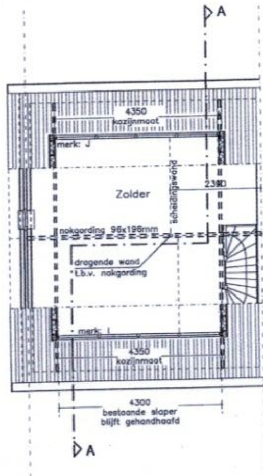
Zolderverdieping
