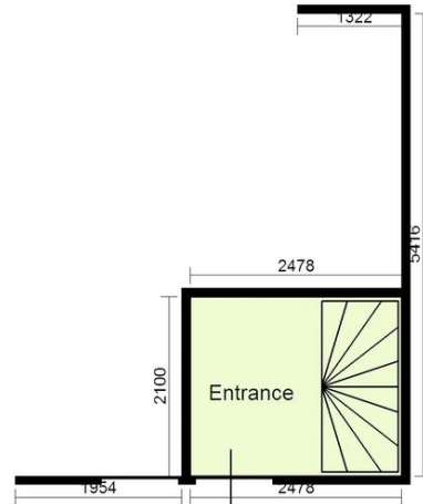
LAMMERMARKT 148 LEIDEN 1st floor
